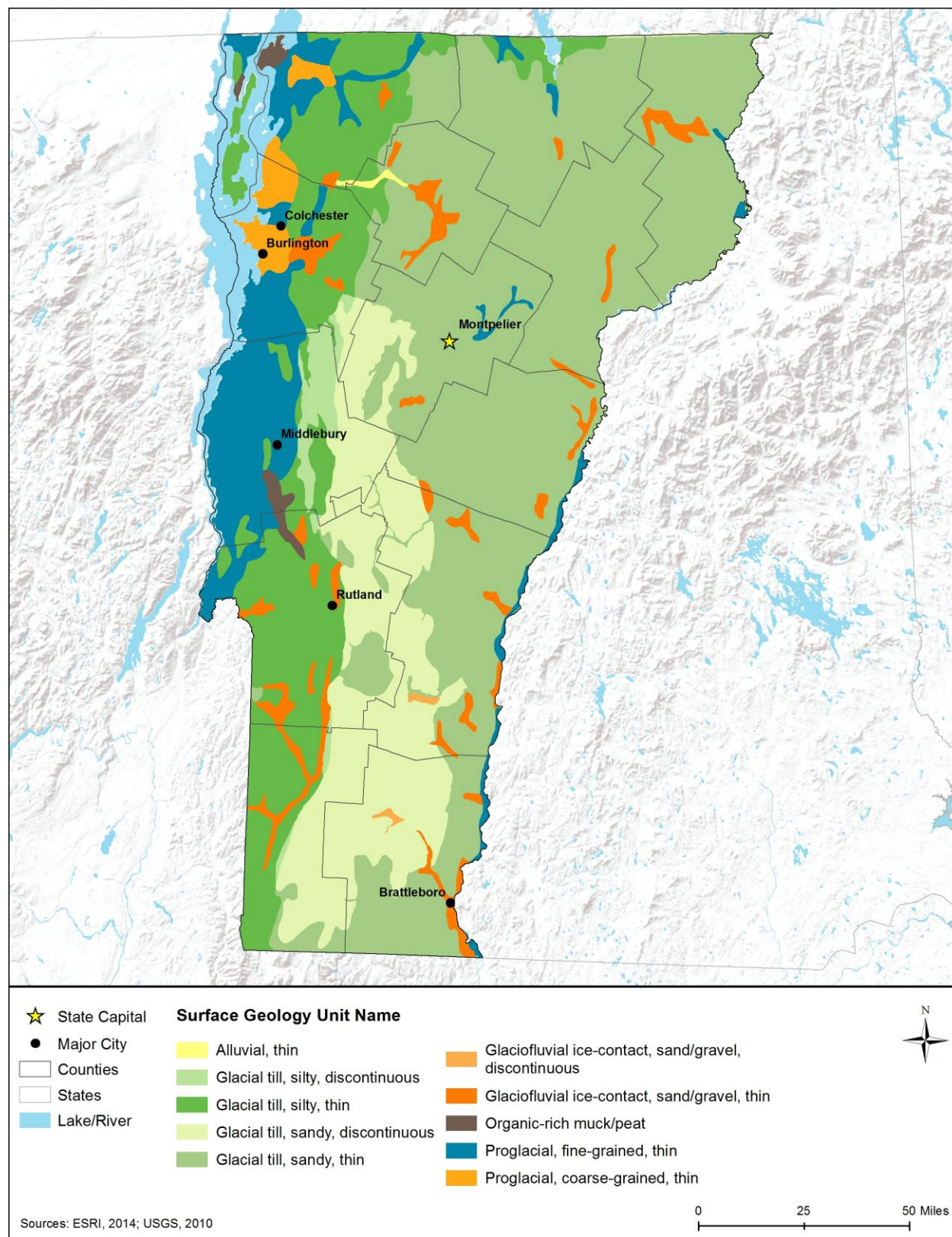
Figure 14.1.3-2: Generalized Surface Geology for Vermont
