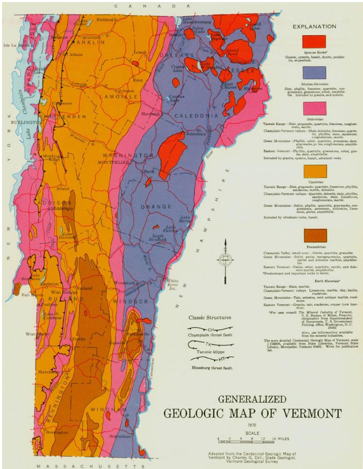
Figure 14.13-3: Generalized Bedrock Geology for Vermont
