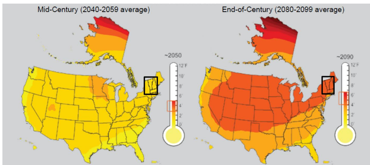
Figure 14.2.14-1: Vermont Low Emission Scenario Projected Temperature Change
