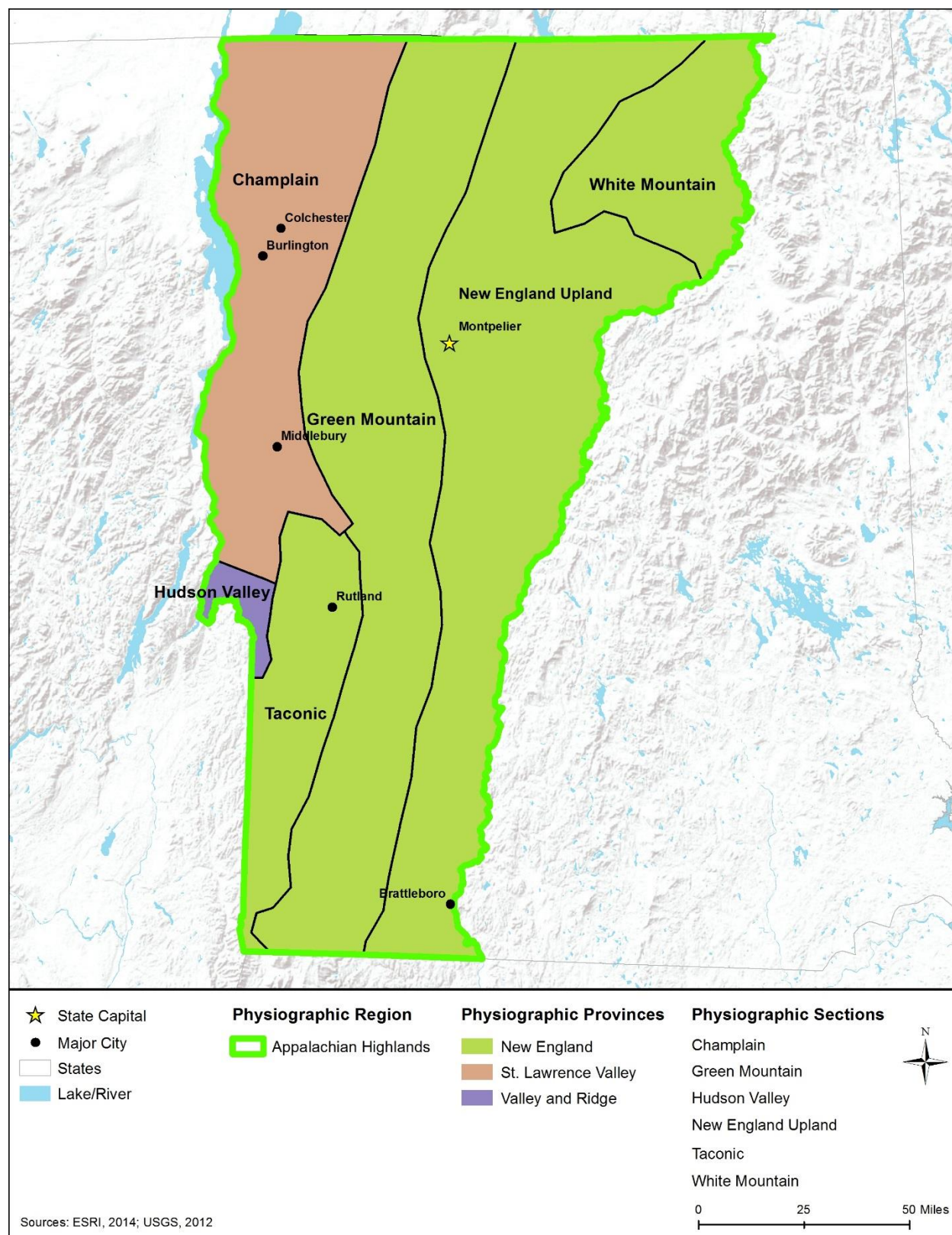
Figure 14.1.11-1: Vermont Physiographic Regions
